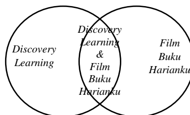
Gambar 2.4 Diagram Venn Keterkaitan Variabel Penelitian
